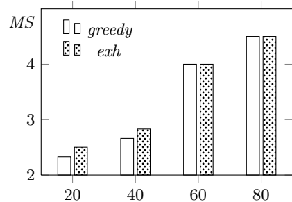
(a) varying n
