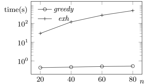
(a) varying n
