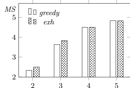
(b) varying k
