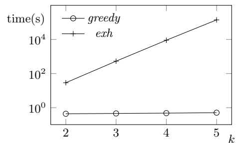
(b) varying k
