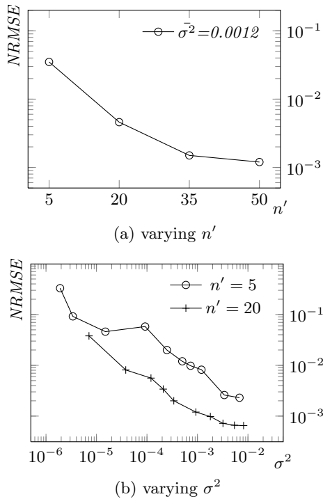
Figure 4: Accuracy of distance metric learning
